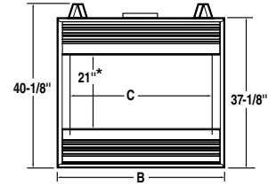
Louvered-Face Front
