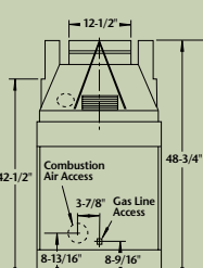
Closed End View
