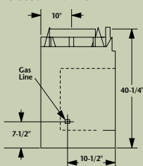
Closed End View
